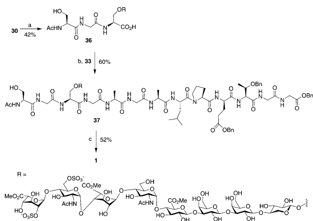
Scheme 5. Reagents and conditions: a) 1. Zn, CuSO 4 (sat.), Ac 2 O/THF/HOAc (2:3:1); 2. NH 2 NH 2 ·H 2 O, HOAc, CH 2 Cl 2 /MeOH (1:1); 3. SO 3 -Et 3 N, DMF, 55 °C; (4) H 2 , Pd/C, CH 2 Cl 2 /MeOH (1:1); 5. NaOMe, MeOH, pH = 9.5; b) HATU, 2,4,6-collidine, DMF; c) 1. H 2 , Pd/C, CH 2 Cl 2 /MeOH (1:1); 2. LiOH, CH 3 OH/H 2 O (1:1), pH = 9.5.
